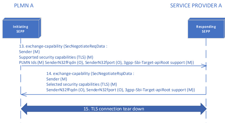
Figure 46 - N32s-c Handshake
