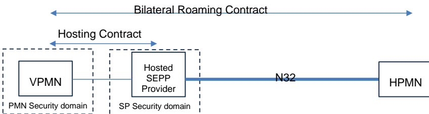
Figure 15 - Bilateral scenario with Hosted SEPP providers
