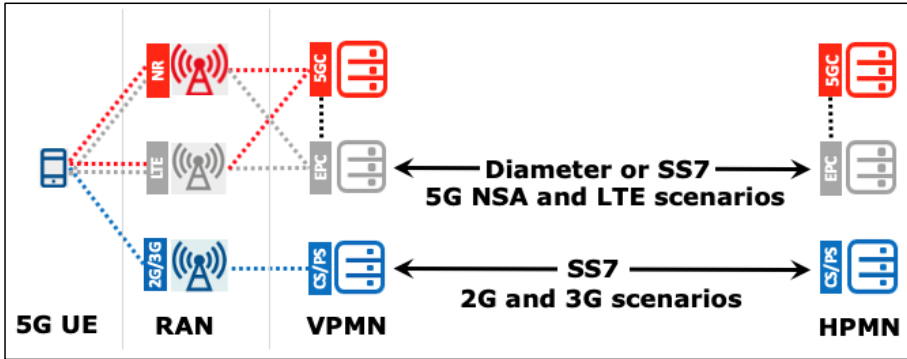
Figure 37 – Least Protected Roaming Traffic Scenarios
