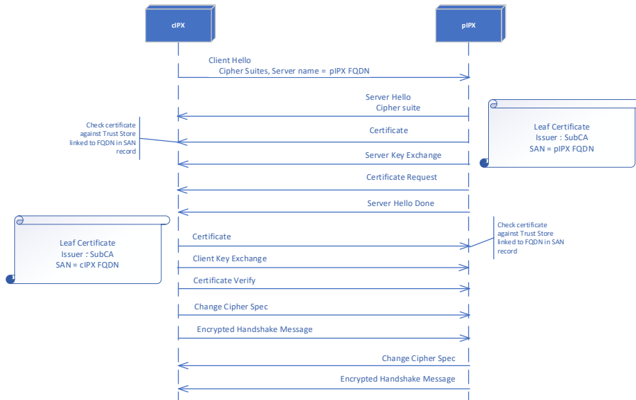
Figure 58 - TLS Connection Setup between hubs
