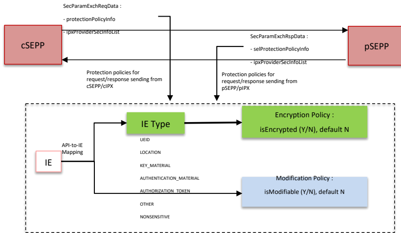
Figure 64 – Illustration of API to IE mapping
