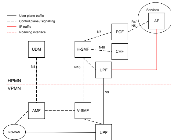
Figure 38 – PCC Architecture with Home Routed Architecture
