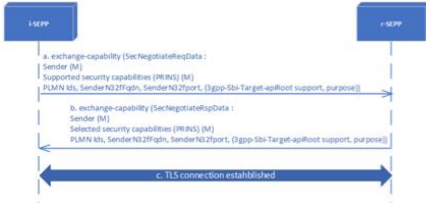
Figure 53 - N32-c Handshake
