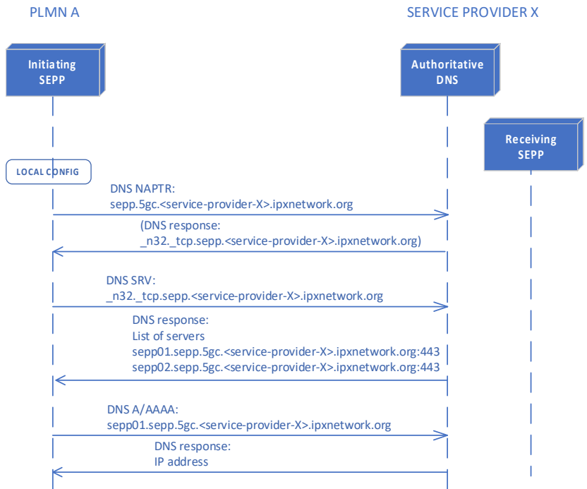
Figure 60 - Dynamic SP SEPP Discovery
