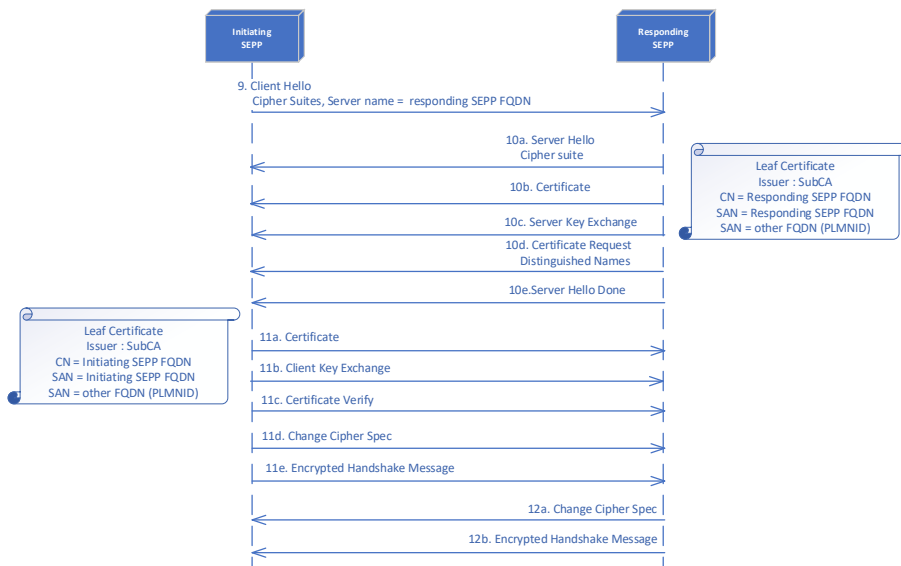
Figure 40 - TLS Handshake
