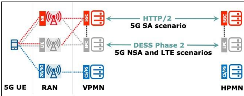
Figure 36 – Confidentiality Protected Roaming Scenarios
