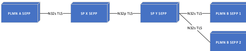
Figure 59 - TLS Hop-by-hop Connections
