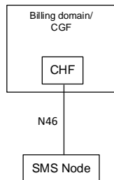
Figure 33 – 5G Reference point Representation (SMS charging)
