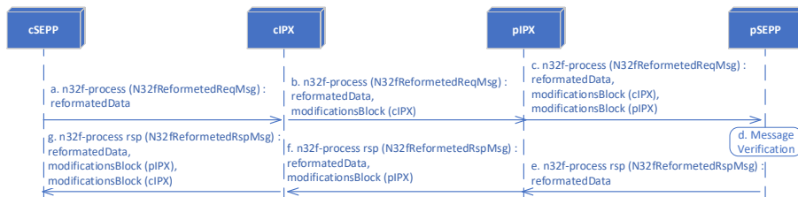
Figure 57 – N32-f Forwarding and Patching
