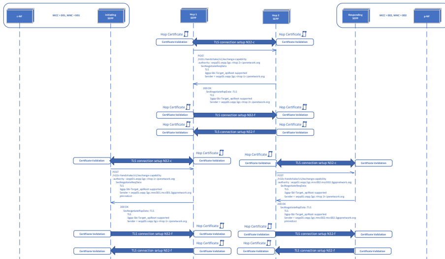
Figure 62 - E2E Connectivity establishment
