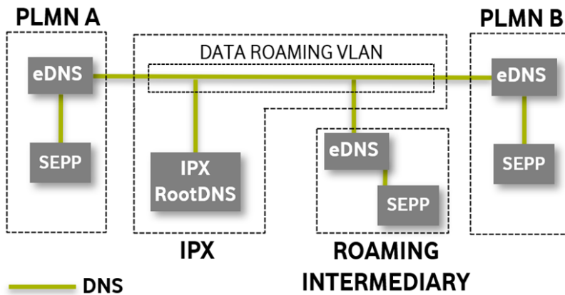
Figure 24– Data roaming VLAN overview.
