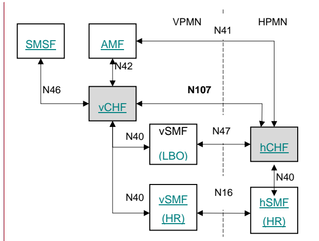
Figure 6 – 5G Reference point Representation (charging)
