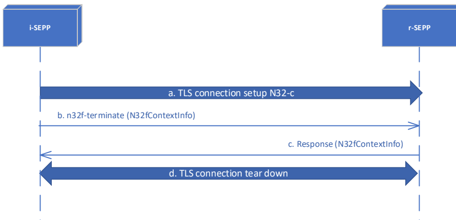
Figure 56 - N32-f Context Termination
