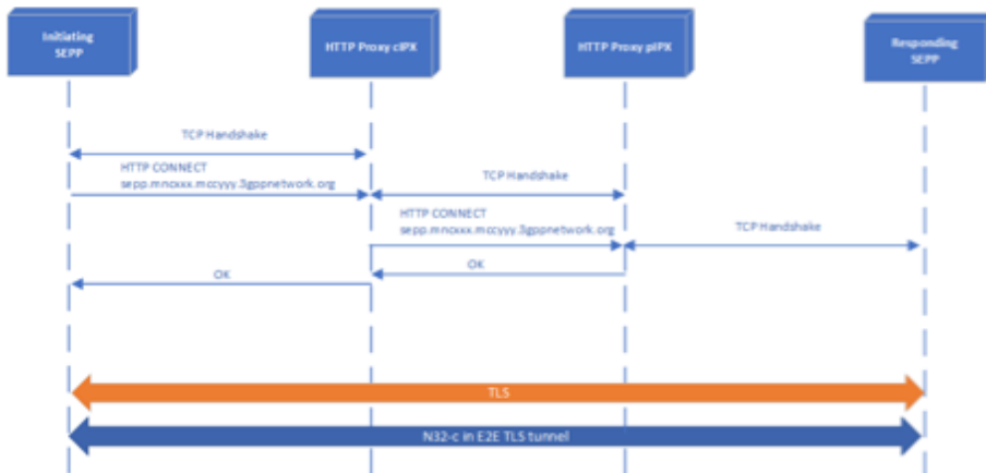
Figure 50 - N32-c mTLS connection using HTTP CONNECT
