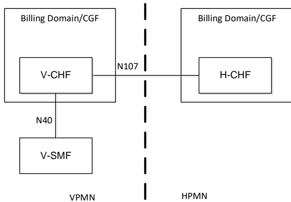
Figure 31 – 5G Reference point Representation (data LBO charging)
