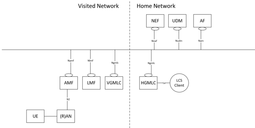
Figure 29 – 5G location detailed architecture (service based)
