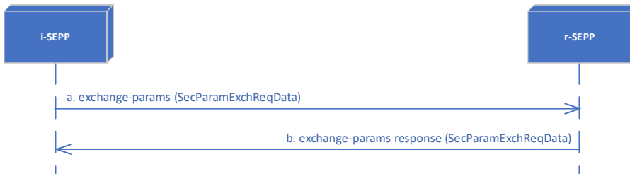
Figure 54 - N32-c Parameter Exchange
