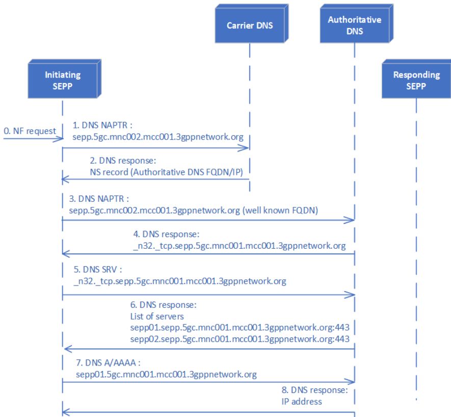
Figure 39 - Dynamic SEPP Discovery
