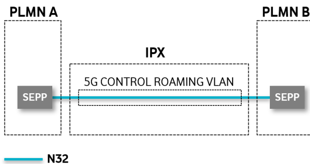
Figure 7 5G control roaming VLAN overview
