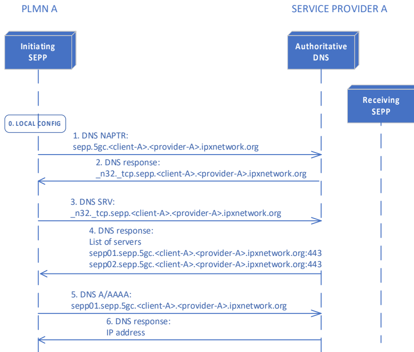
Figure 44 - Dynamic SEPP Discovery of Hosted SEPP
