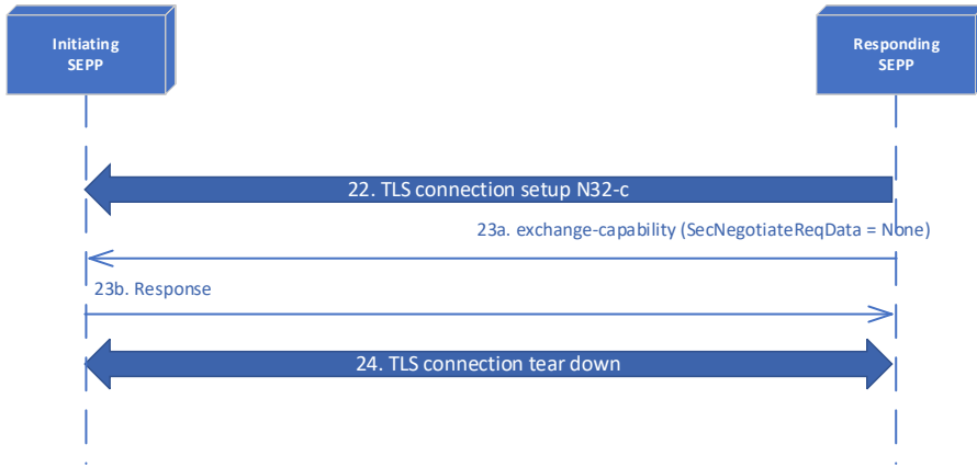
Figure 43 - N32 connection termination
