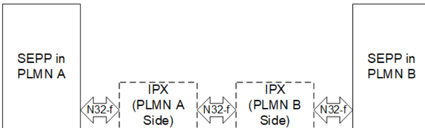
Figure 10 – N32-f Interface with PRINS (ALS)
