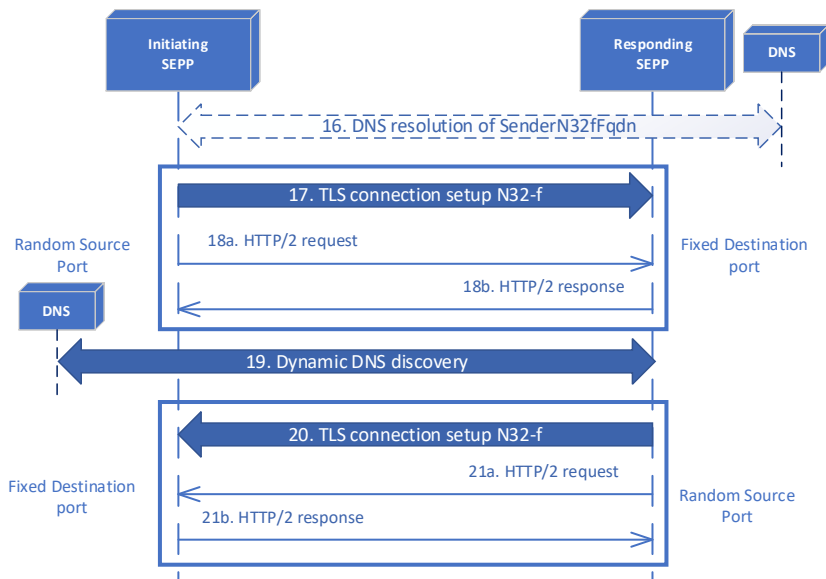
Figure 42 - N32-f connection establishment
