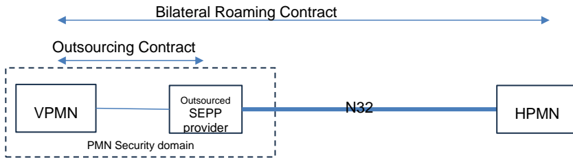
Figure 14 - Bilateral scenario with Outsourced SEPP provider
