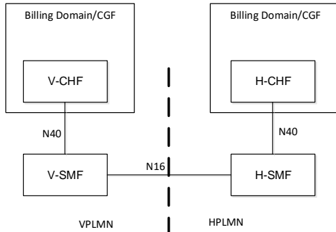
Figure 30 – 5G Reference point Representation (data HR charging)
