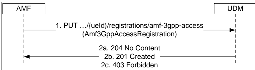
Figure 27 – AMF Registering for 3GPP access [10] Section 5.3.2.2.2
