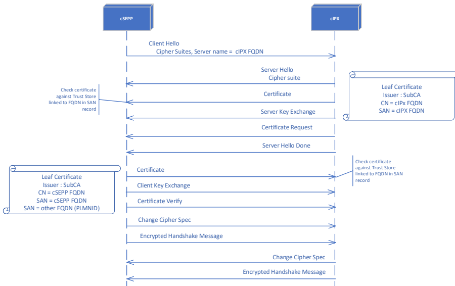
Figure 52 - N32-f mTLS connection establishment
