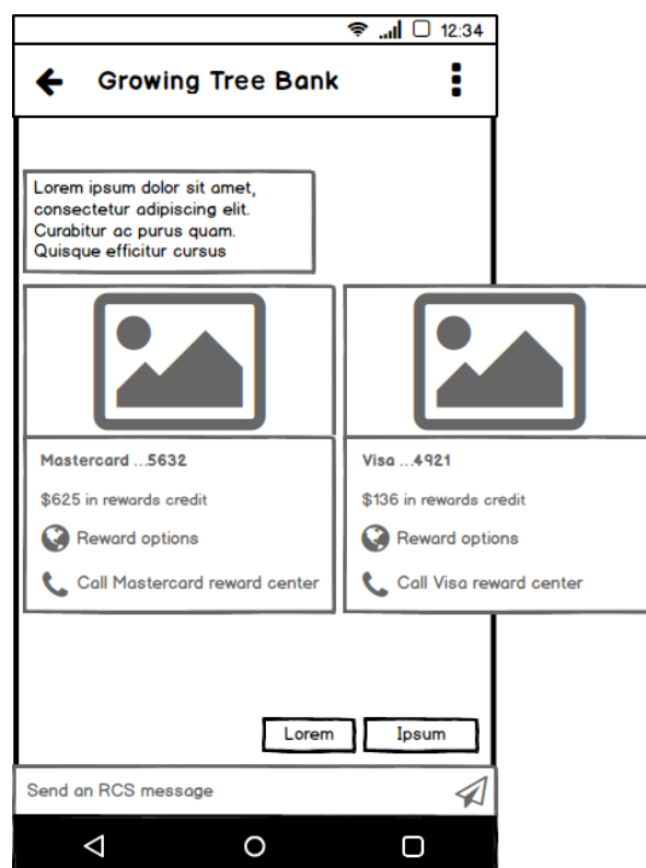
Figure 6: Rich Card Carousel example
