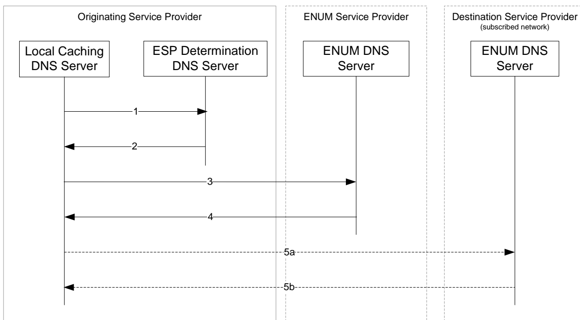
Figure 15: Example ENUM resolution in the Multiple Root Model
