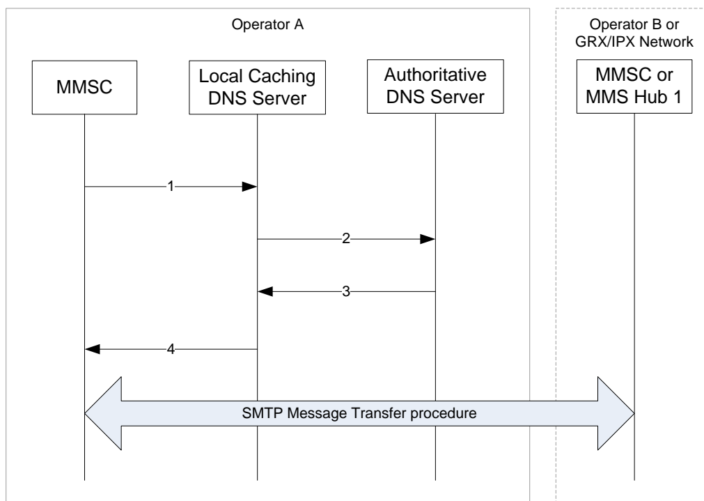
Figure 10: MMS Inter-operator Delivery
