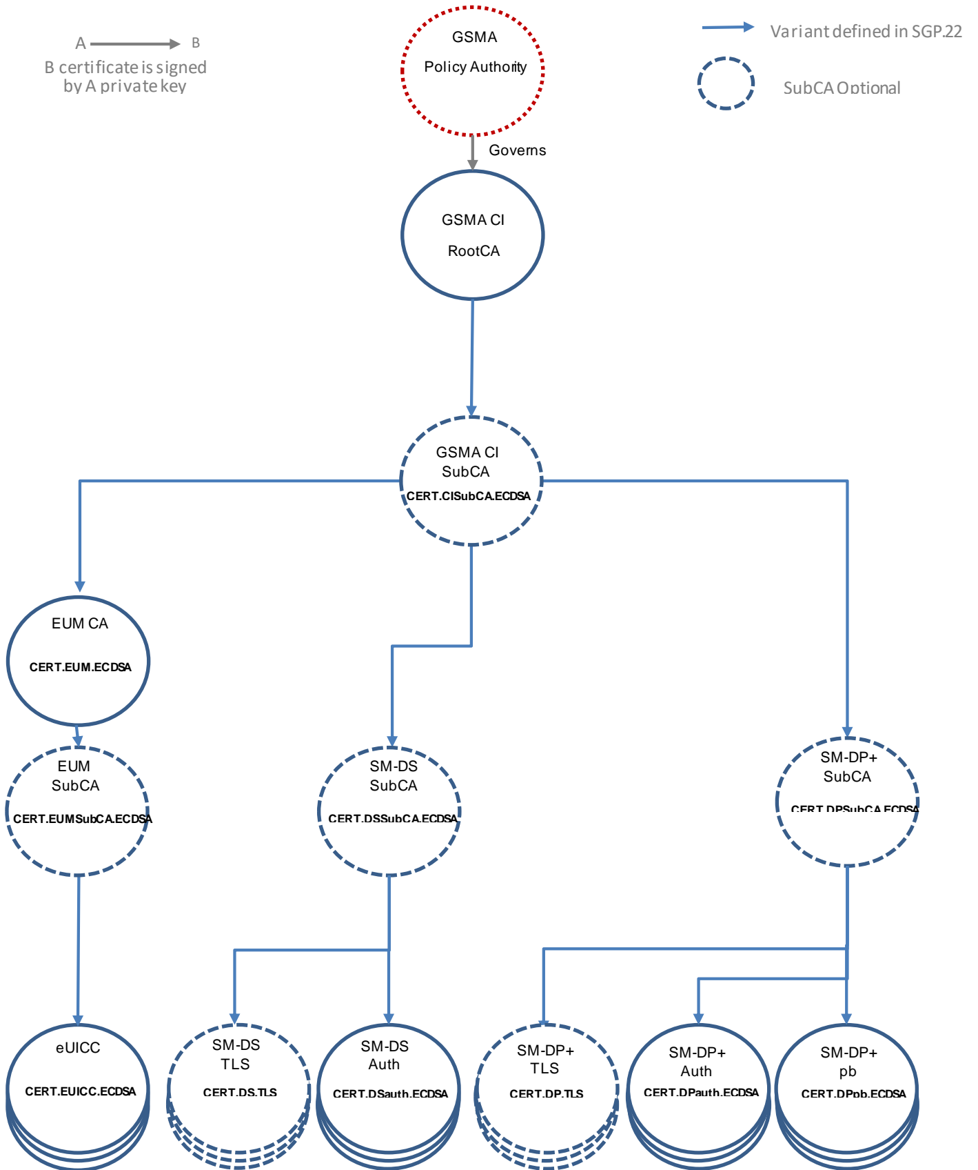
Figure 2 Certificate chain for SGP.22 [11]
