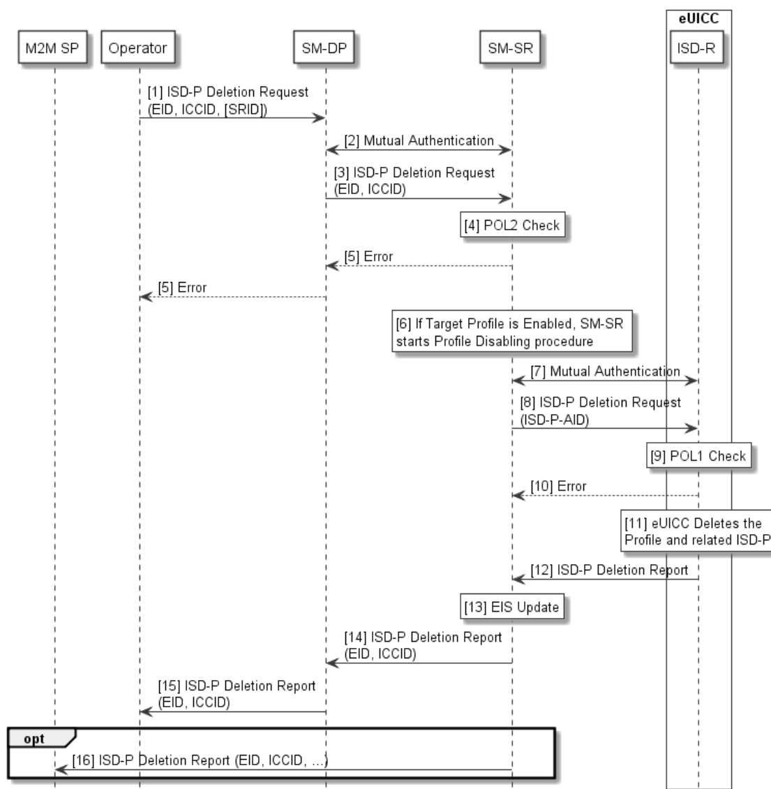
Figure 12: Operational Profile Deletion via SM-DP
