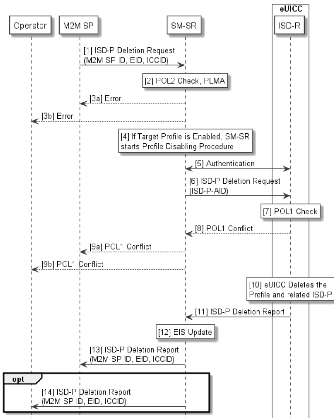
Figure 20: ISD-P Deletion via M2M SP
