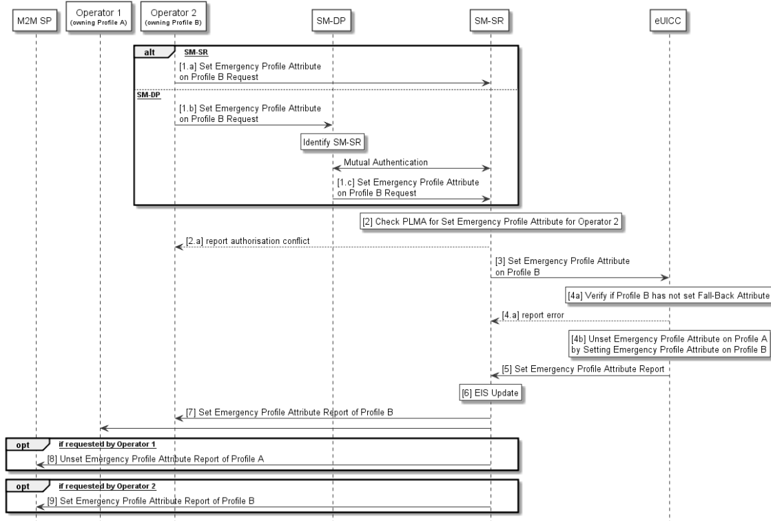
Figure 24: Emergency Profile Attribute Management (case 2)
