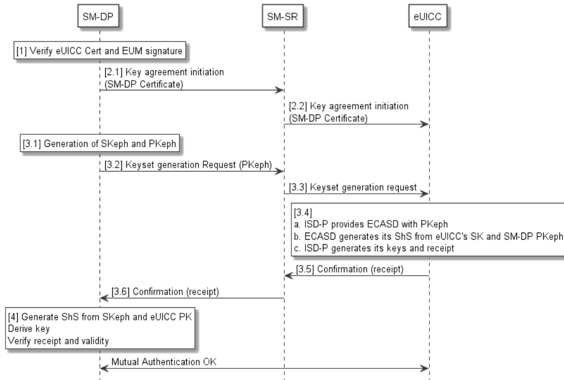
Figure 32: ElGamal Key Agreement
