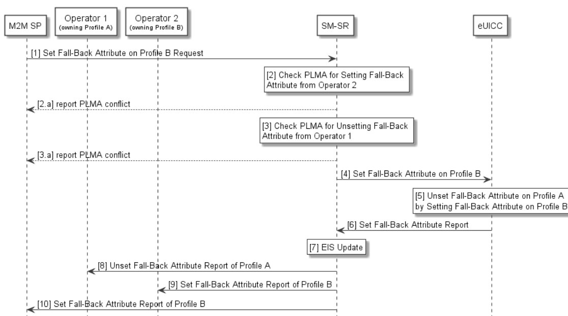
Figure 22: Fall-Back Attribute Management via M2M SP
