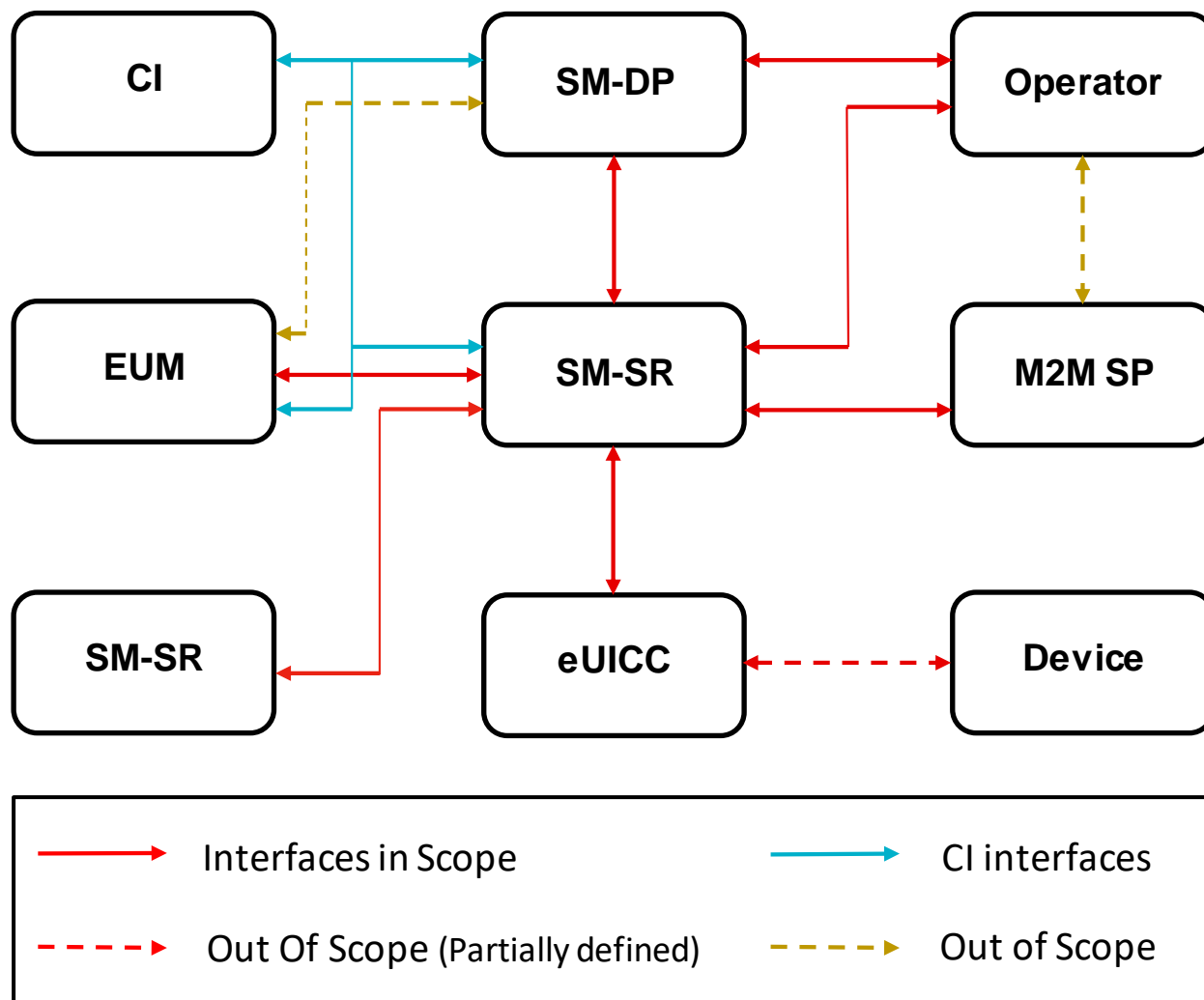
Figure 1: eUICC Remote Provisioning System
