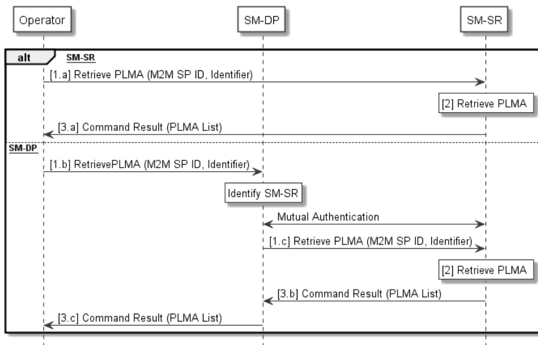
Figure 15: Retrieve Profile Lifecycle Management Authorisation by Operator
