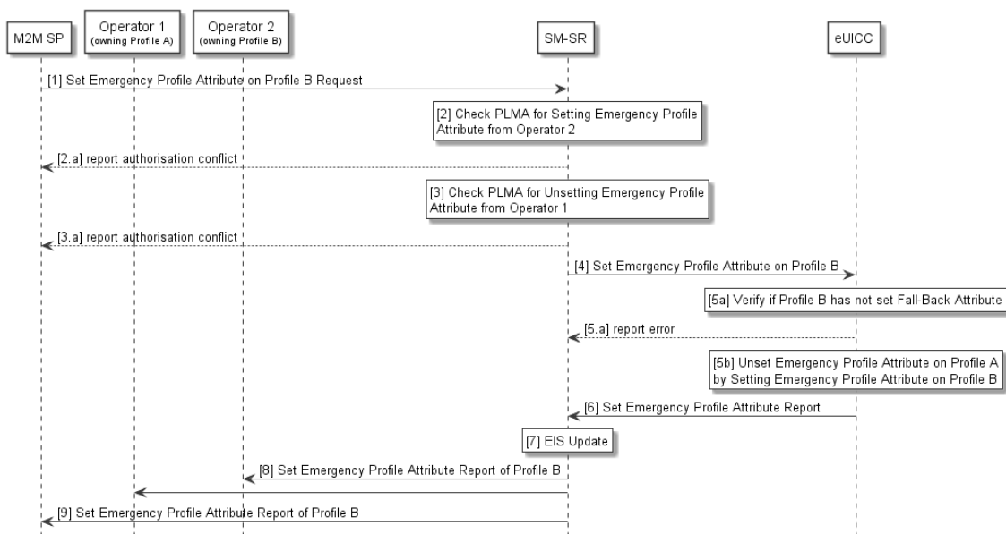
Figure 26: Emergency Profile Attribute Management via M2M SP (case 2)
