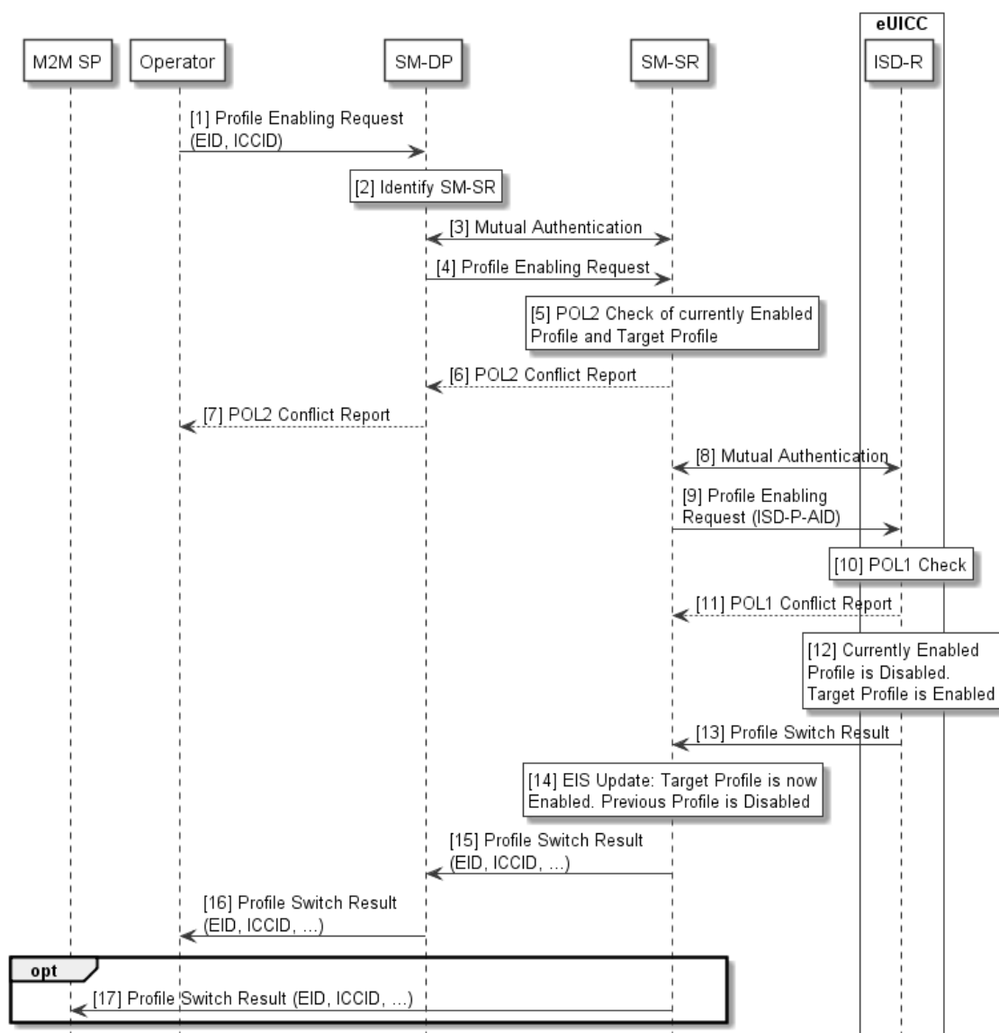
Figure 9: Profile Enabling via SM-DP
