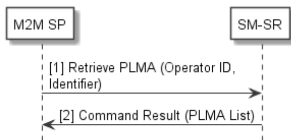
Figure 16: Retrieve Profile Lifecycle Management Authorisation by M2M SP Start Condition:
