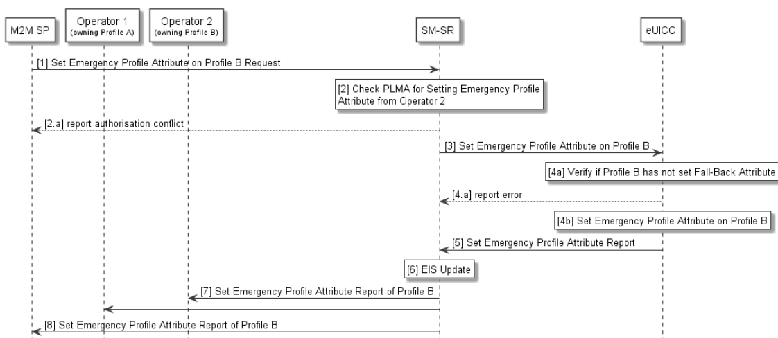
Figure 25: Emergency Profile Attribute Management via M2M SP (case 1)
