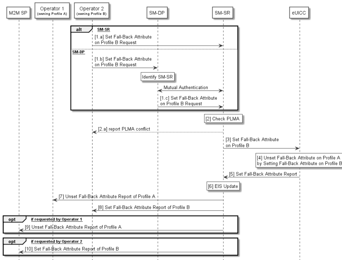
Figure 21: Fall-Back Attribute Management
