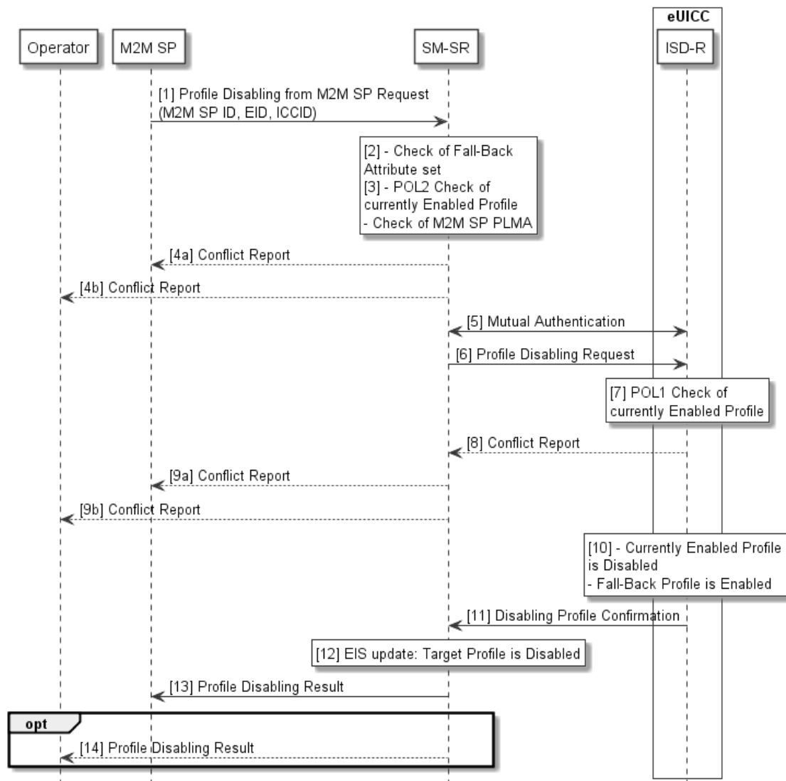
Figure 19: Profile Disabling via M2M SP
