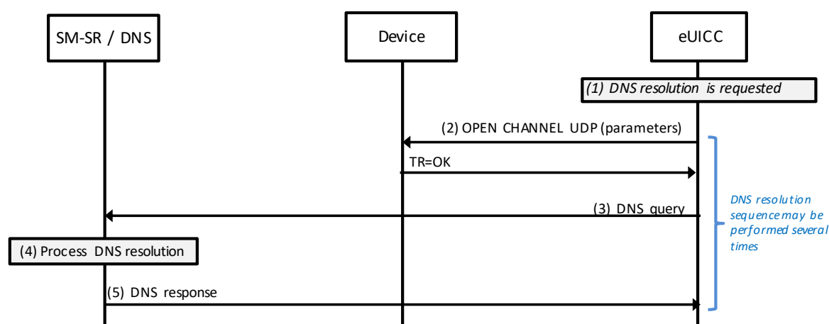
Figure 10: Sequence for Basic DNS resolution
