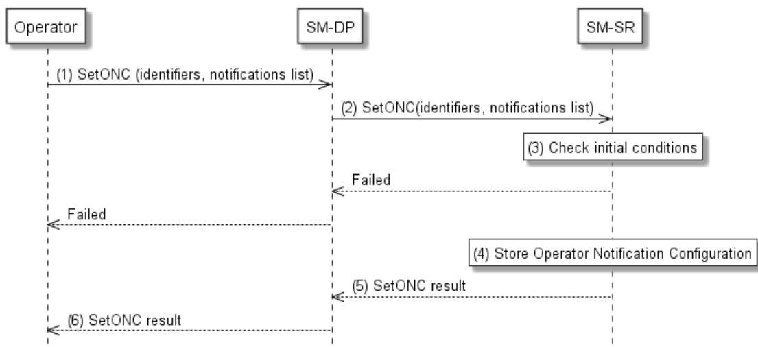
Figure 42: Set Operator Notification Configuration via SM-DP
